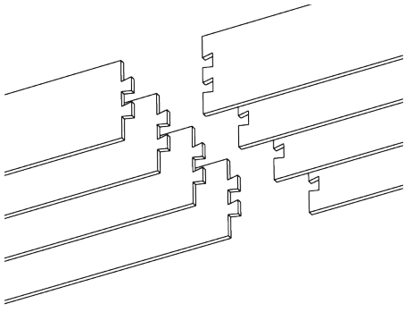
DOVETAIL JOINT
