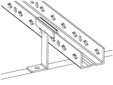
U-PROFILE SUSPENSION
